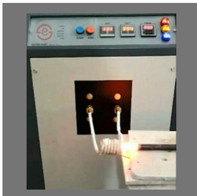
Induction Bar End Heater
